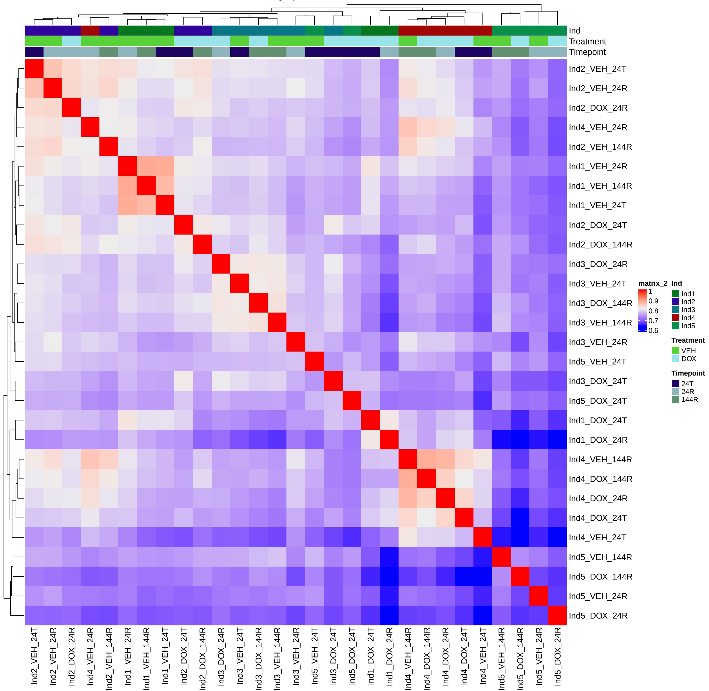
Filtered log2cpm H3K27me3
